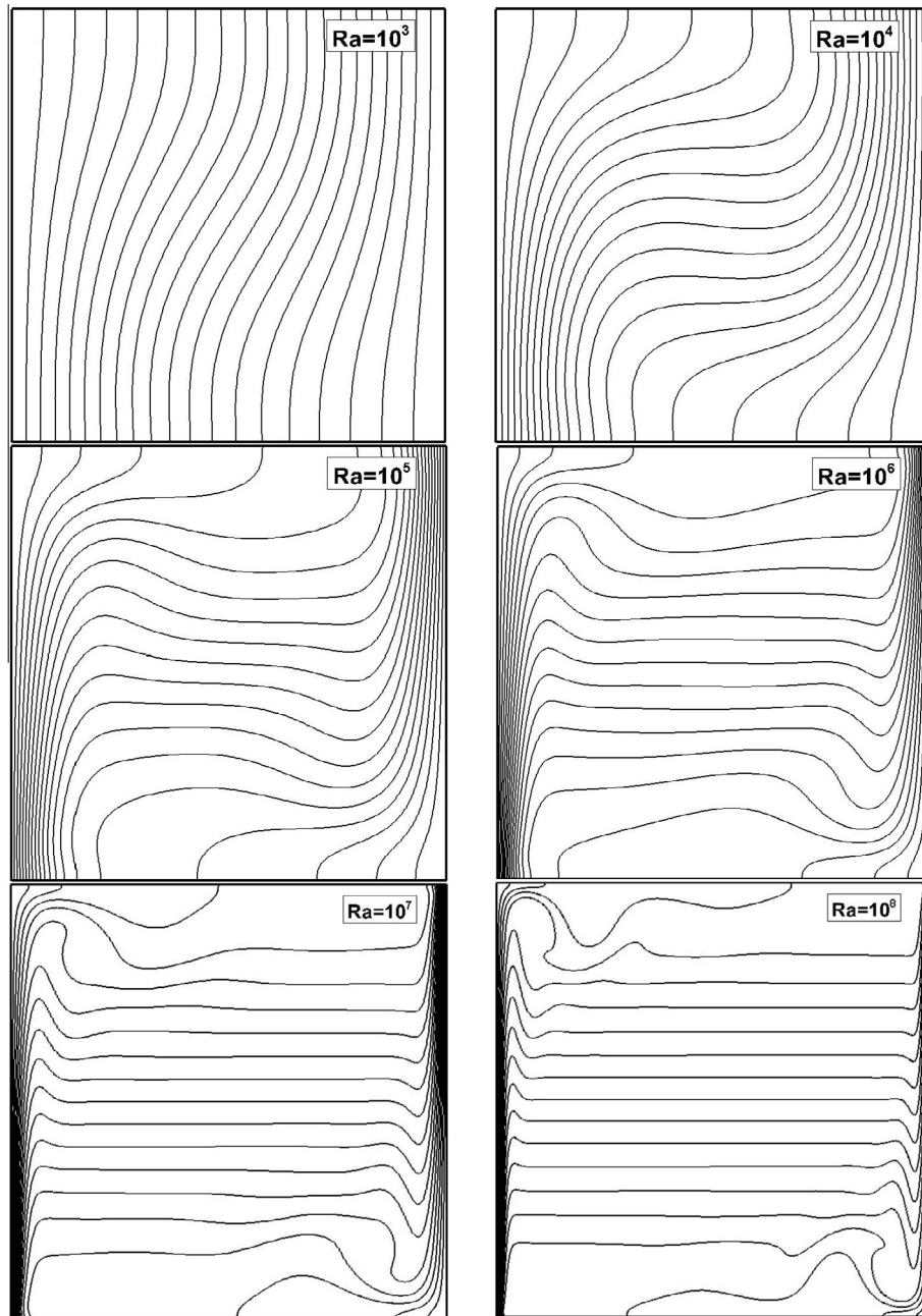
Fig. 5. Isotherms at different Rayleigh numbers.
