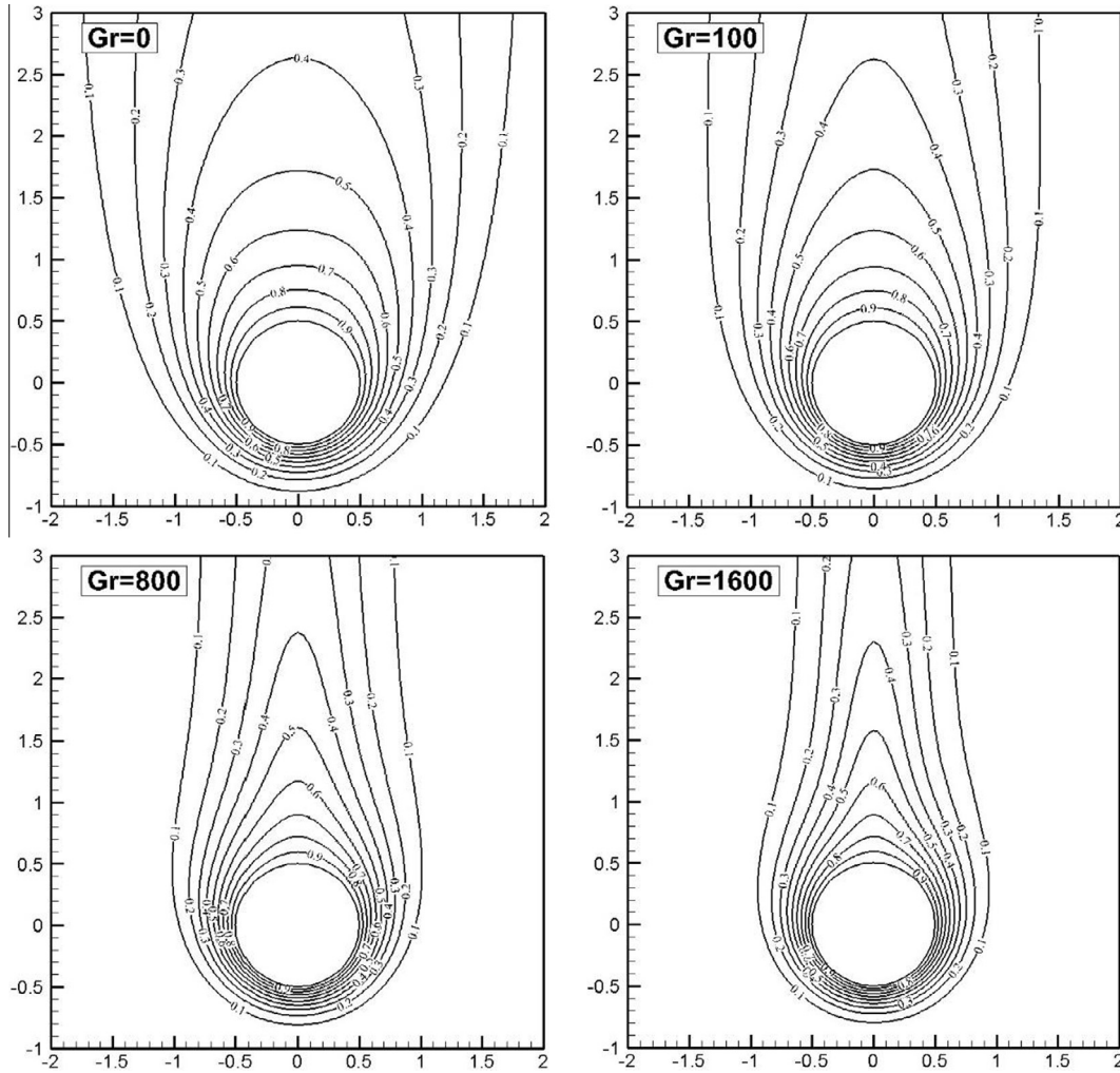
Fig. 10. Isotherms of mixed heat transfer system at Re = 20 for different Grashof numbers.
