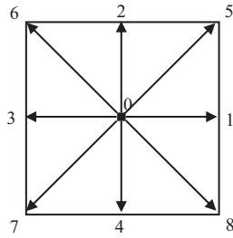
Fig. 1. Illustration of the D2Q9 model.
