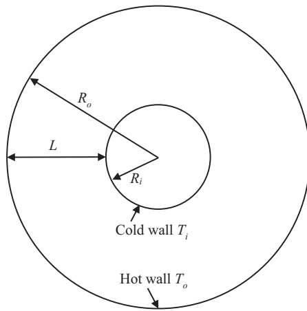
Fig. 6. Illustration of the setup for natural convection in a concentric annulus.
