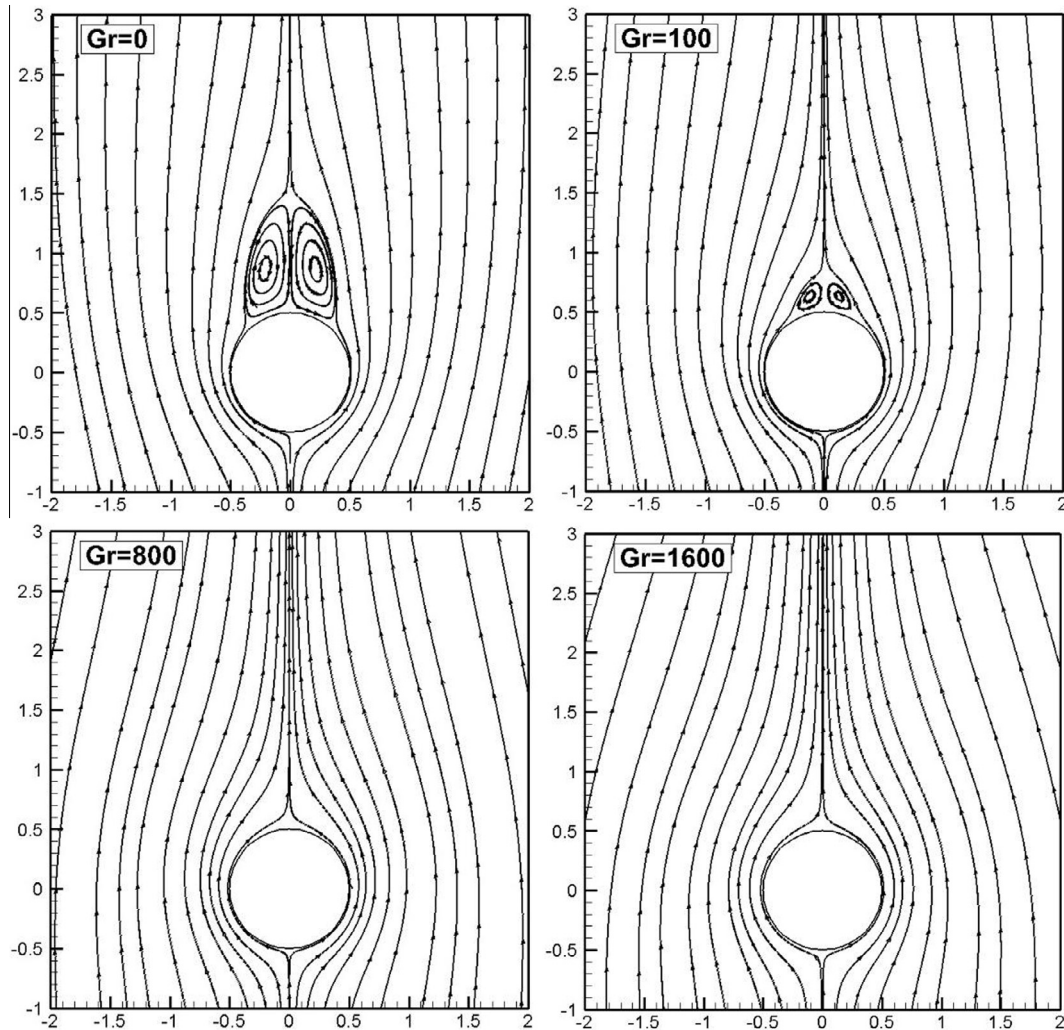
Fig. 9. Streamlines of mixed heat transfer system at Re = 20 for different Grashof numbers.
