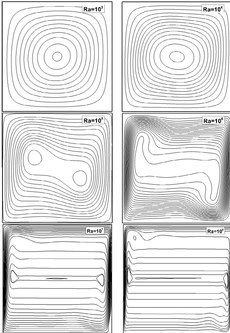
Fig. 4. Streamlines at different Rayleigh numbers.
