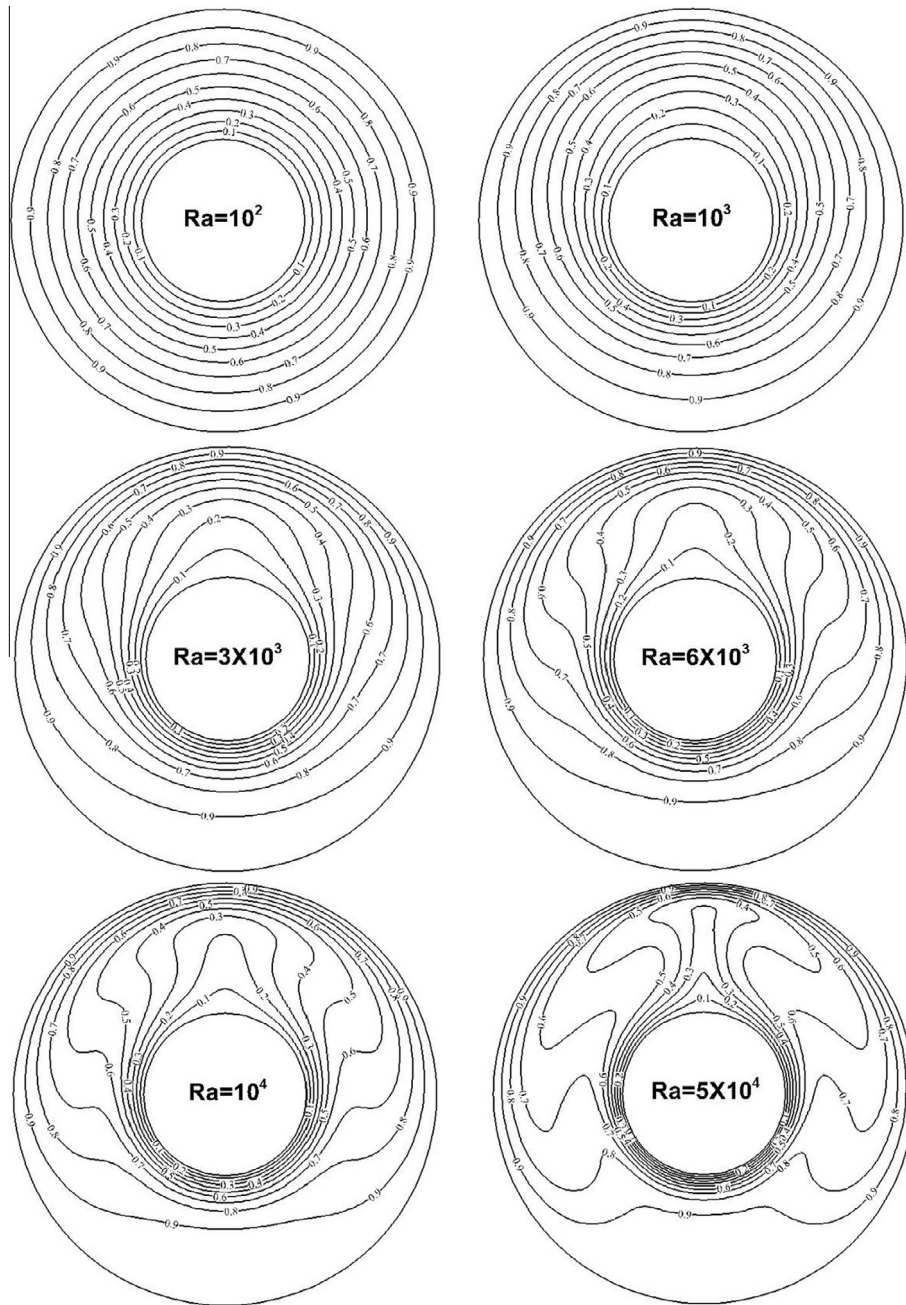
Fig. 7. Isotherms at different Rayleigh numbers.
