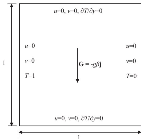
Fig. 2. Physical configuration of the setup for 2D natural convection in a square cavity.
