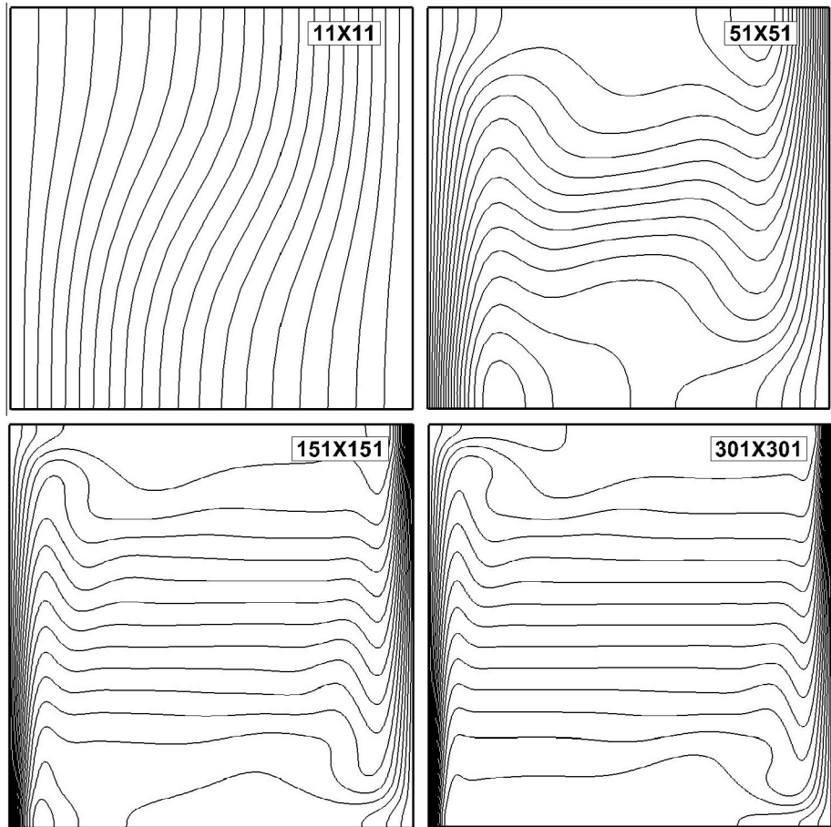
Fig. 3. Isotherms for different mesh sizes at Ra = 10^6 .
