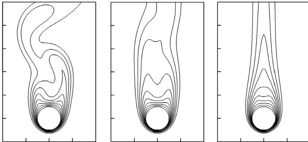
Fig. 12. Isotherms of mixed heat transfer at Re = 100 and different Richardson numbers. From left to right: Ri = 0, 0.1 and 0.5 .
