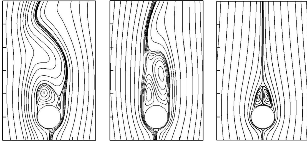
Fig. 11. Streamlines of mixed heat transfer at Re = 100 for different Richardson numbers. From left to right: Ri = 0, 0.1 and 0.5 .
