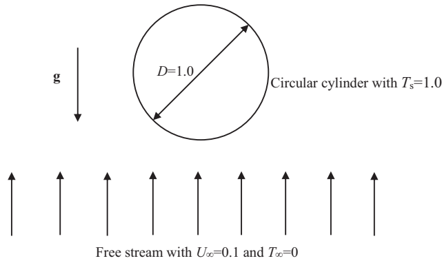
Fig. 8. Illustration of the mixed heat transfer simulation setup from a heated circular cylinder.
